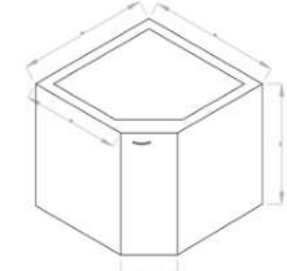
Model DHLTS - 04 900X900X750X900
